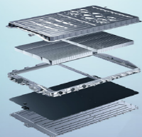
CELL-TO-BODY BATTERY
